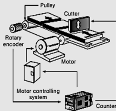
[Diameter of the Pulley connected with the encoder is 22mm, pulse number of encoder per 1revolution:1000]
